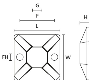
MB3-MB5 (plan view)
