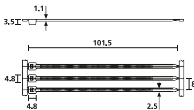
T18RA型卷盘
