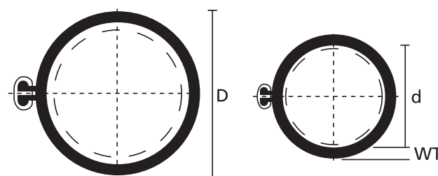
Split Heatshrink Repair Kit - Dimensions.
