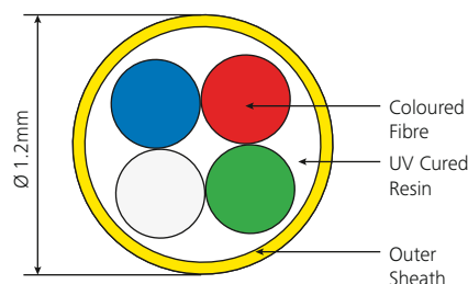
4 Fibre Cable Cross Section.
