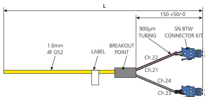
Cable Configuration.
