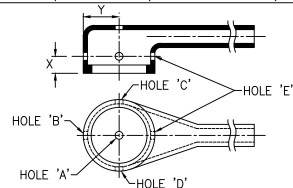
OPTIONS TO STANDARD PART FILLER PORT/DRAIN HOLES (CODES P, D AND P1)
