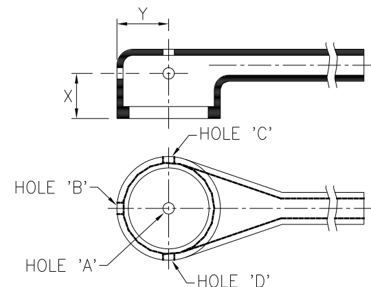
OPTIONAL FILLER PORT/DRAIN HOLES DETAIL
