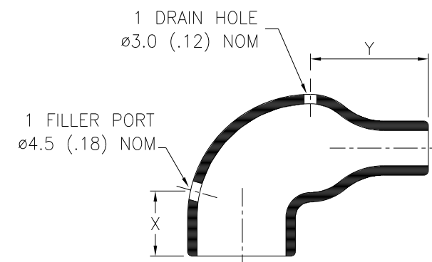
OPTION TO STANDARD PART FILLER PORT (CODE P)
