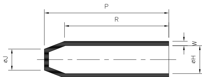
STANDARD PART (AFTER UNRESTRICTED RECOVERY)
