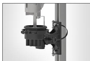
FRBU 16P Mobra Mounting Bracket (detail).
