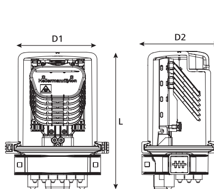
Front view of Small Length CFN Closure with SE-IR Trays.
