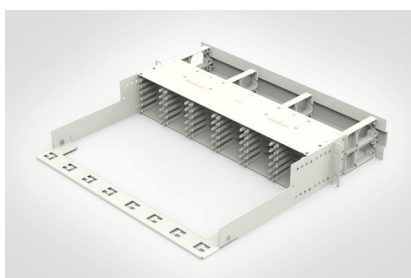
RapidNet ULTRA8 2U (rear view).
