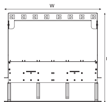
RapidNet ULTRA8 (top view).
