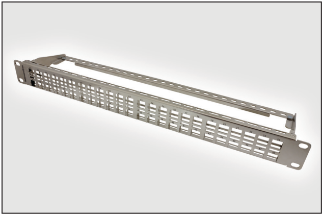
Modular 1U 48 Port Patch Panel (shown with cable manager)
