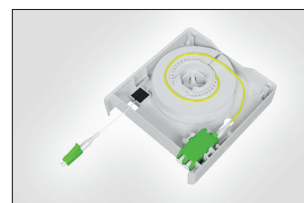
Internal view of the Faint Fibre Outlet with fibre spool, LC DX adaptor and connector.
