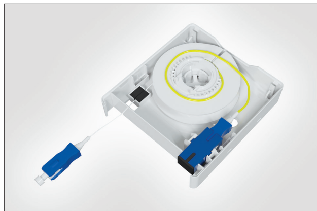
Internal view of the Faint Fibre Outlet with fibre spool, SC SX adaptor and connector.
