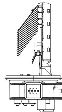
Side view of Small Length CFN Closure with SC-B Trays
