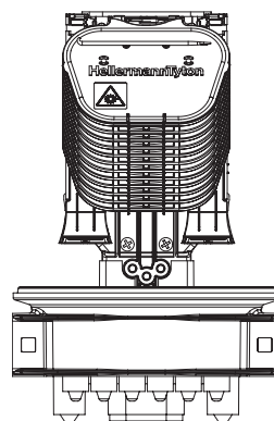
Front view of Small Length CFN Closure with SC-B Trays
