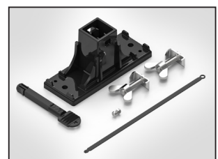
CFN Mobra Mounting Bracket pictured.
