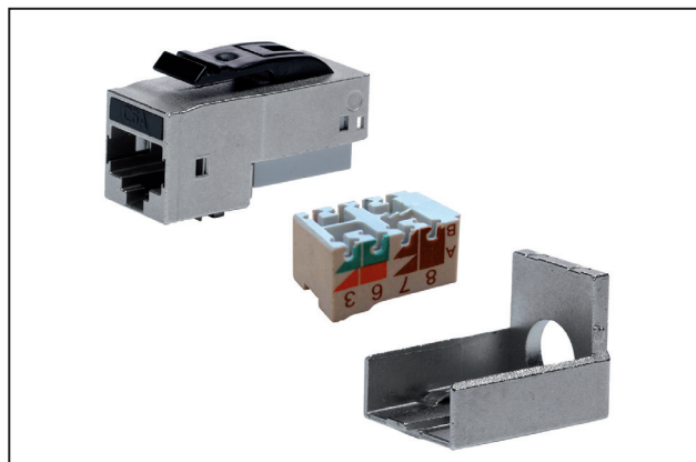
Category 6A Keystone Jack
