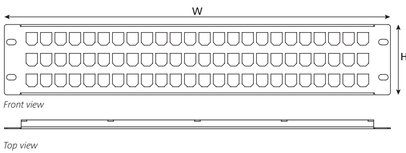
2U 72 Port
