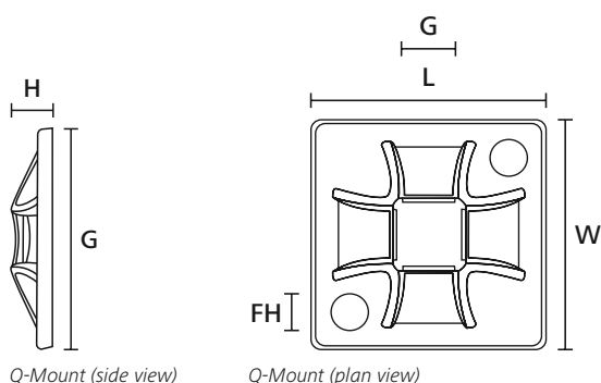
Q-Mount (side view)
