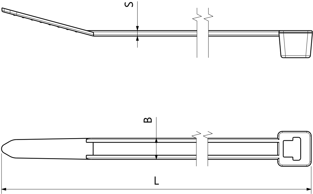
Cable tie T50R
