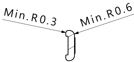
Section View A-A Scale 3:1
