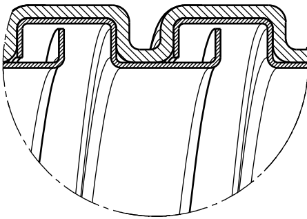
Detail X (Prinzip/principle)
