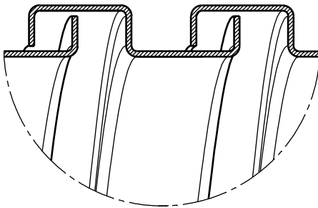
Detail X (Prinzip/principle)
