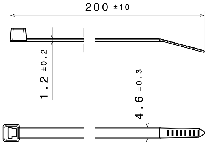
T50R Delivery condition:Unassembled set
