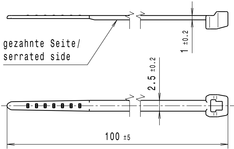
Lieferzustand / Delivery condition Kabelbinder T18ROS / Cable tie T18ROS 2:1
