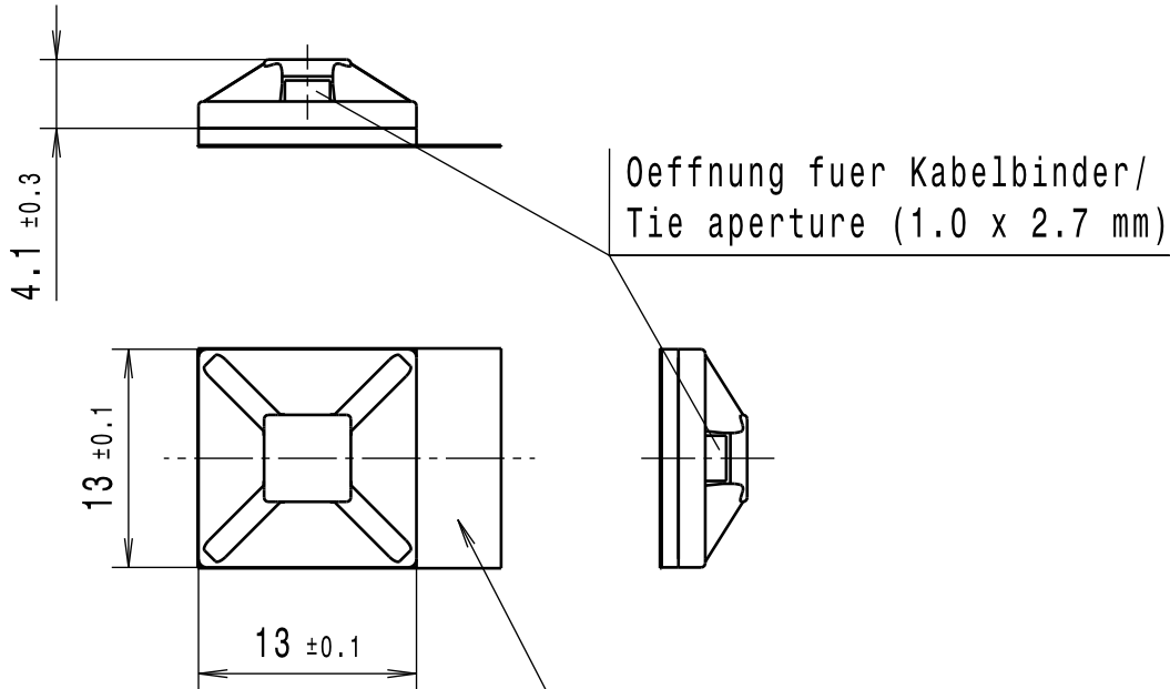
Lieferzustand / Delivery condition Sockel MB2APT / Socket MB2APT 2:1
