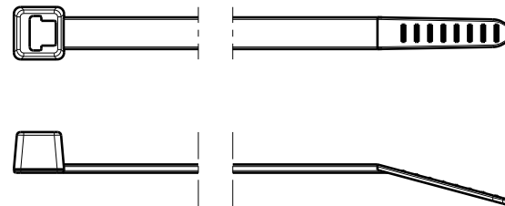
T50R DELIVERY CONDITION: UNASSEMBLED SET
