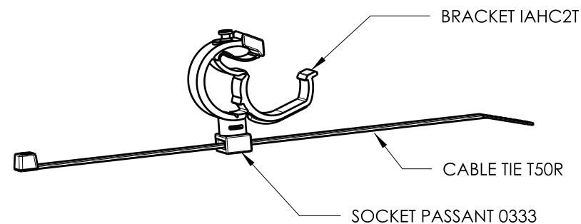
ISOMETRIC VIEW ASSEMBLY EXAMPLE SCALE 1:2
