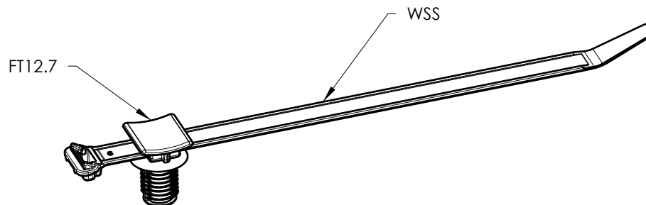
ASSEMBLED EXAMPLE VIEW SCALE 1:2
