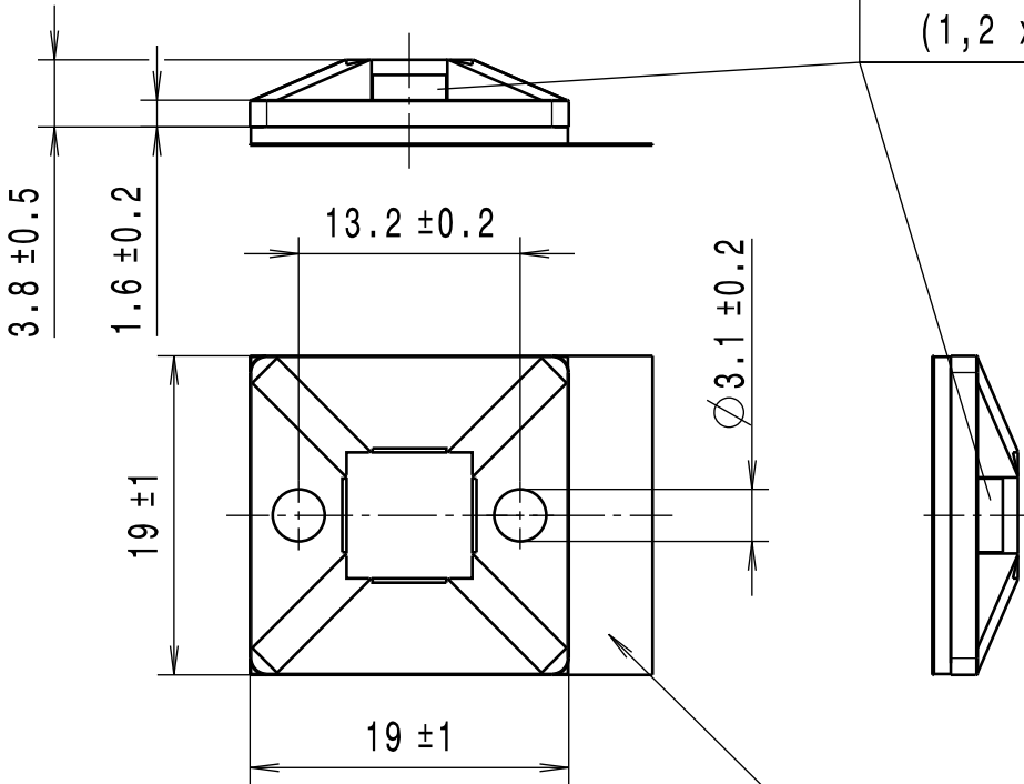
Lieferzustand / Delivery Condition Sockel MB3APT-A / Socket MB3APT-A 2:1
