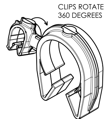
ISOMETRIC VIEW ROTATED
