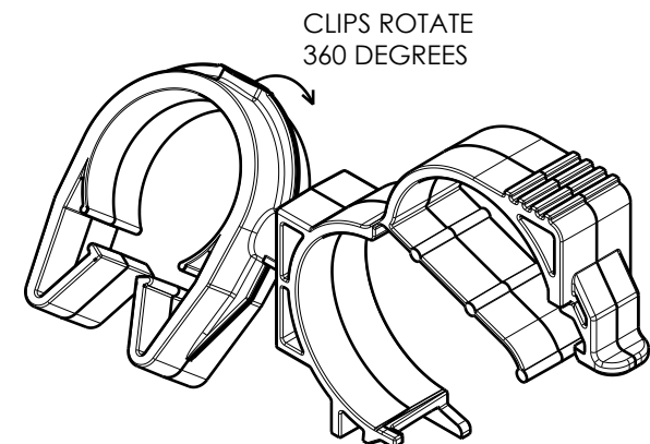
ISOMETRIC VIEW OPEN
