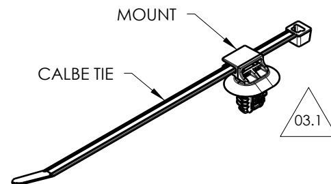
ASSEMBLED EXAMPLE OPTION 2 FOR REFERENCE ONLY SCALE 1:2
