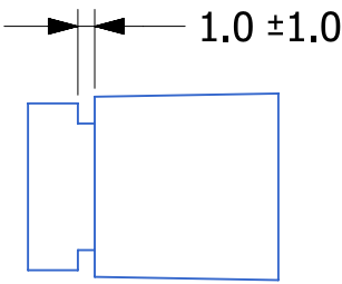
DETAIL A FOR APPLICABLE METAL CLIP TYPES
