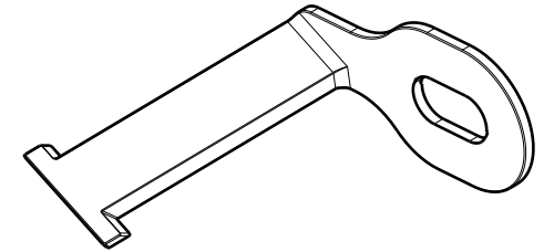
ISOMETRIC VIEW
