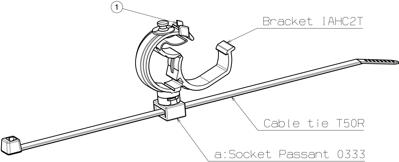
Assembly Example
