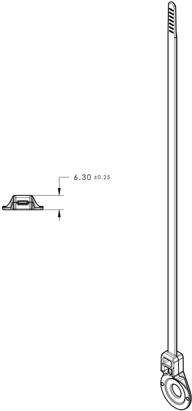
ISOMETRIC VIEW
