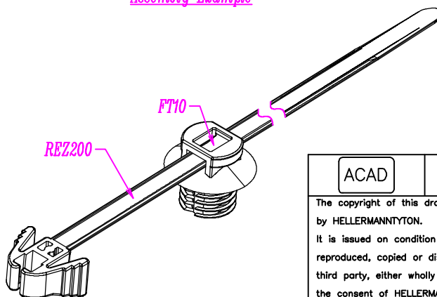
Assembly Example
