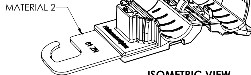
ISOMETRIC VIEW SCALE 1 : 1 PRODUCT SHIPPED IN CLAMP OPEN POSITION
