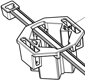
ASSEMBLED EXAMPLE VIEW OPTION 1 MAX TENSION OF 150N
