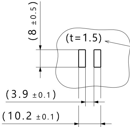
Hole pattern snap hooks / Lochbild Rasthaken 1:1
