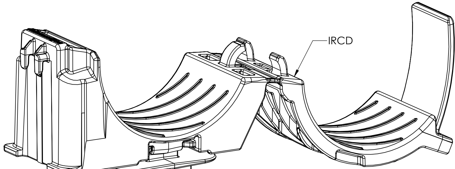
Isometric View SCALE 3 : 2 Product shipped in clamp open position as shown
