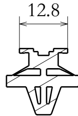
Section View B-B Scale 1:1
