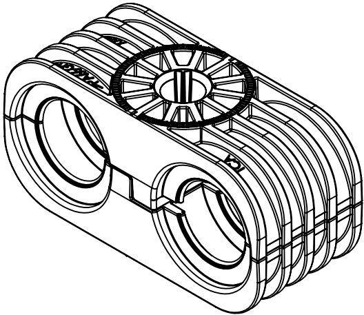
HDCM2A Assembled View
