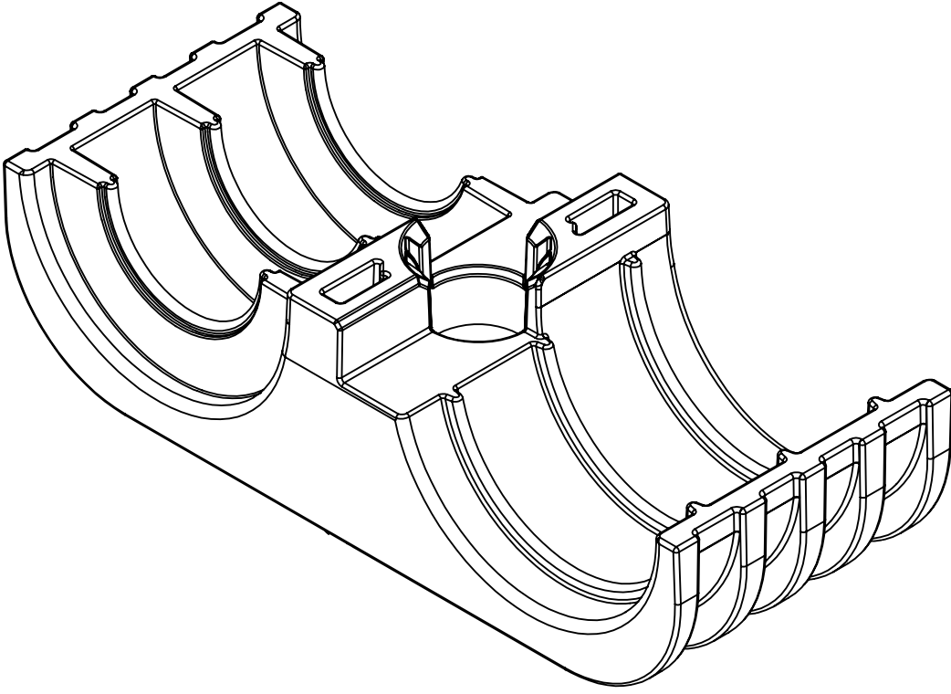
HDCM2D Isometric View SCALE 2 : 1
