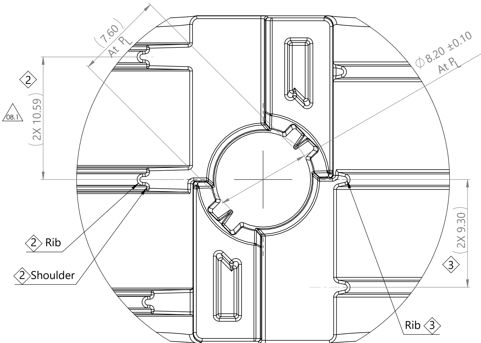
DETAIL A SCALE 5 : 1
