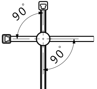
Cable tie position admitted into 90° area 扎带间可以90度旋转
