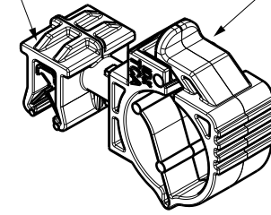
Isometric view Closed position
