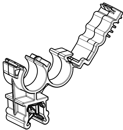
Isometric view 1:1
