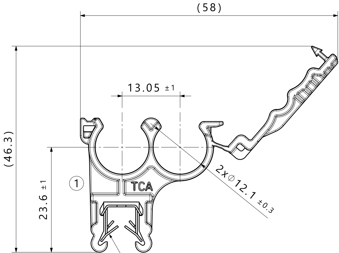
Clamp TE4-799-001-K, fit to material thickness 3-6 mm/ Blechklammer TE4-799-001-K, passend fuer Materialdicke 3-6 mm
