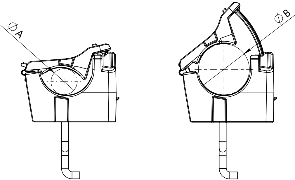
Minimum Bundle Diameter
