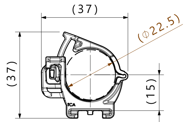
Reference view Closed maximum bundle diameter
