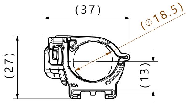
Reference view Closed minimum bundle diameter
