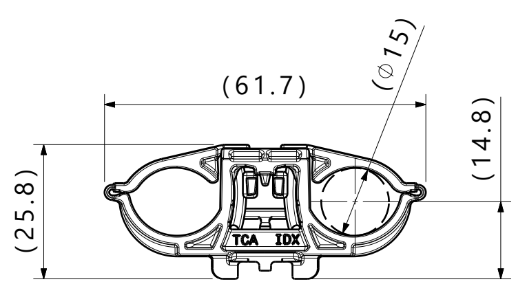
Reference view Closed minimum bundle diameter Scale 1:1
