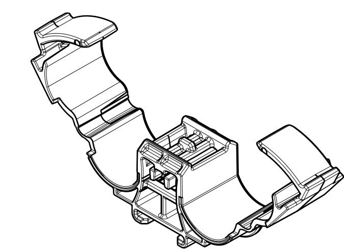
Isometric view Open Scale 1:1
