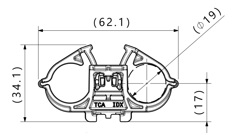
Reference view Closed maximum bundle diameter Scale 1:1
