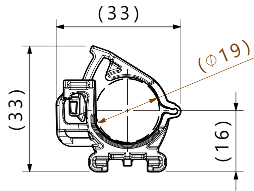
Reference view Closed maximum bundle diameter
