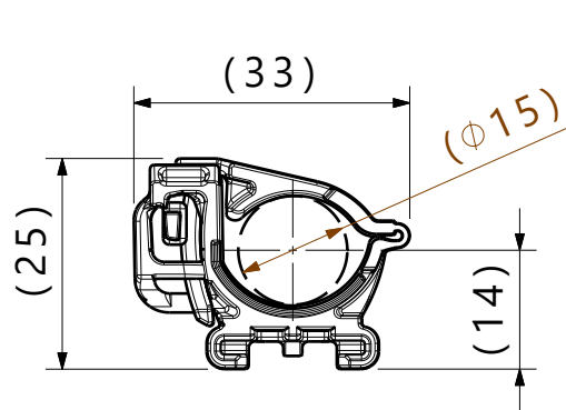
Reference view Closed minimum bundle diameter
