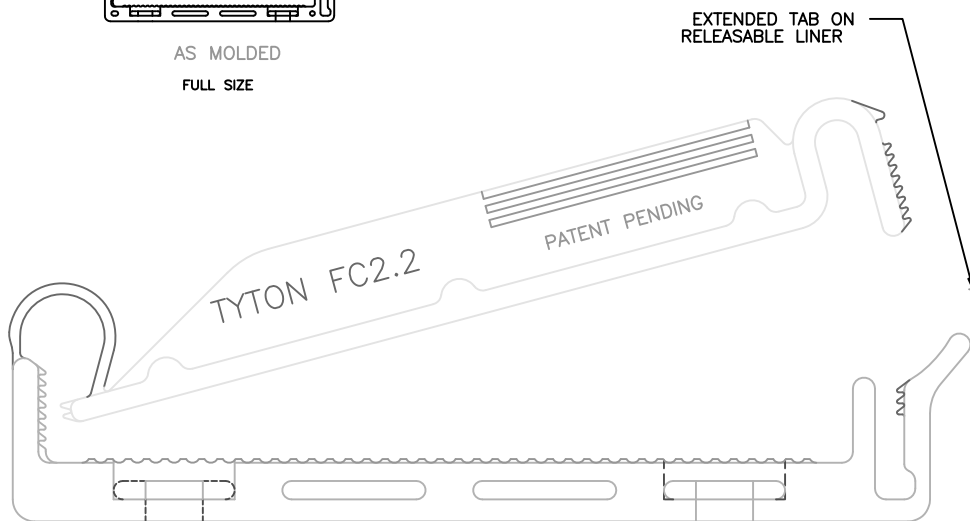
AS MOLDED
